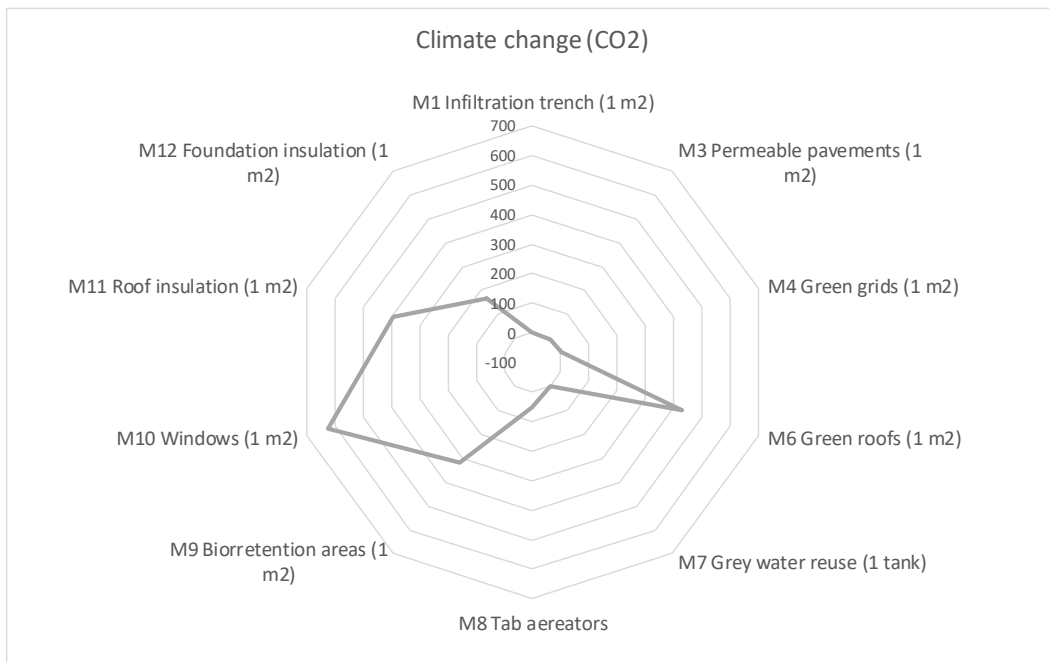
Figure 2: Life Cycle Assessment results per reference unit of the different adaptation measures solutions evaluated for the impact category Climate Change.
